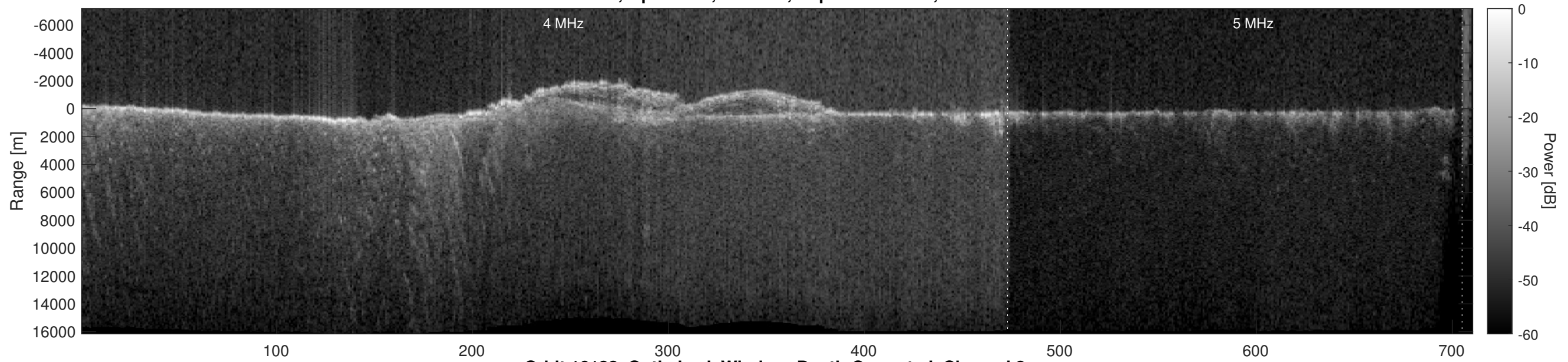
Orbit 16132, Optimized, Window, Depth-Corrected, Channel 2
