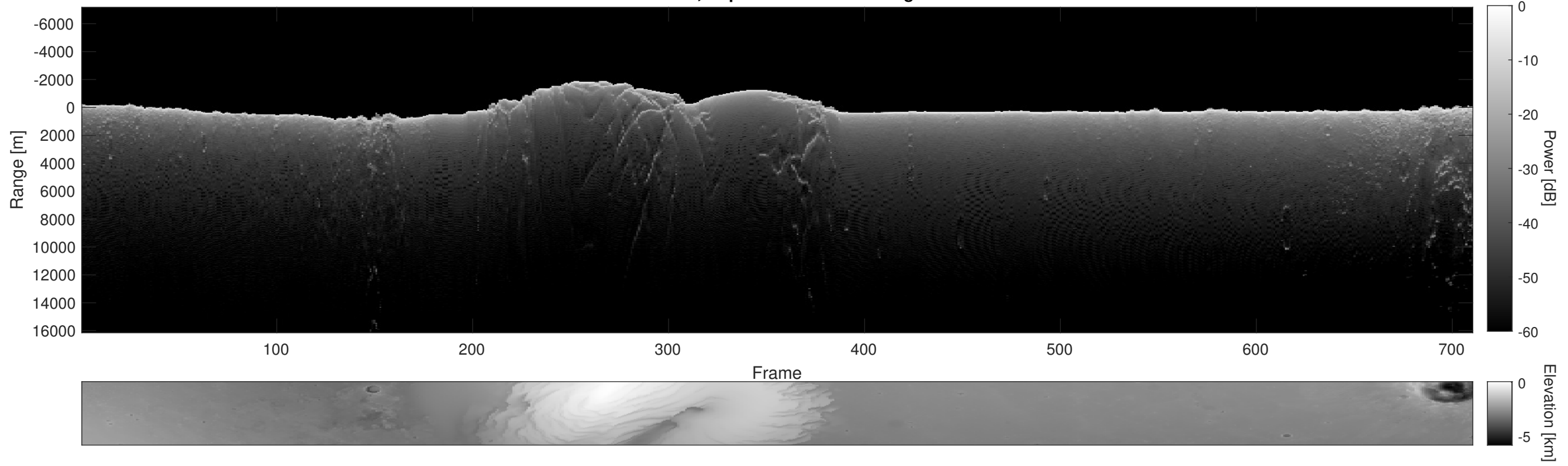
Orbit 16132, Depth-Corrected Cluttergram
