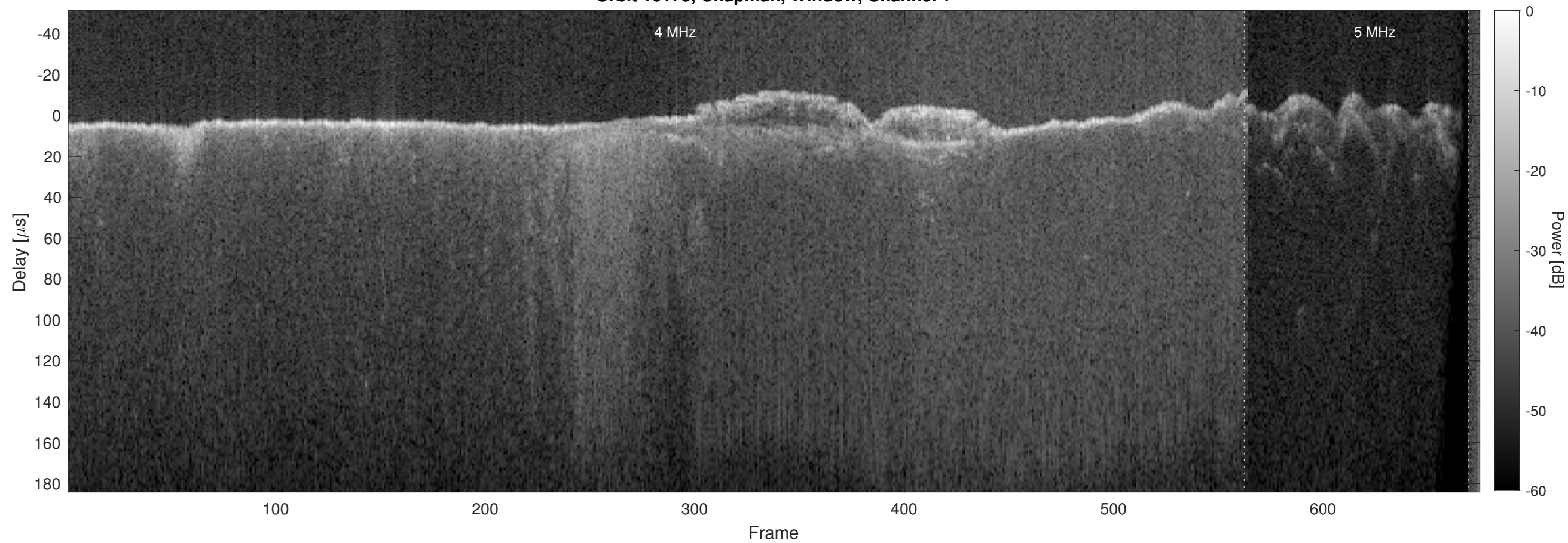
Orbit 16178, Chapman, Window, Channel 2
