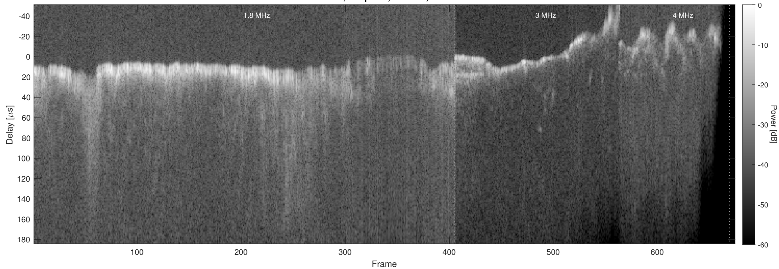
Orbit 16178, Chapman, Window, Channel 2
