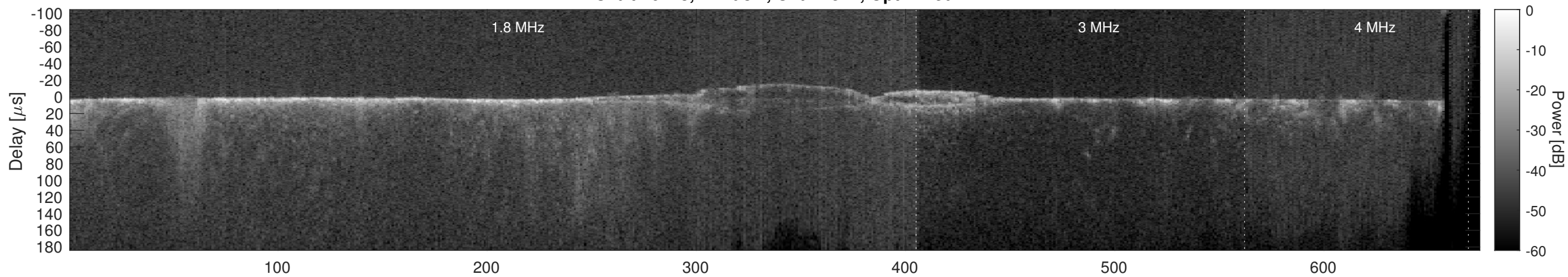
Orbit 16178, Cluttergram
