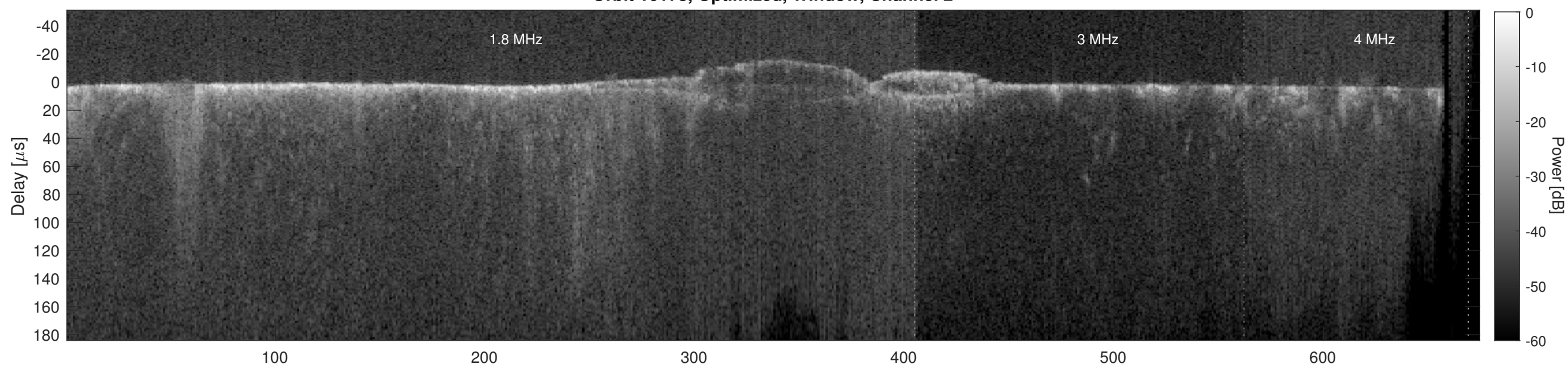
Orbit 16178, Cluttergram
