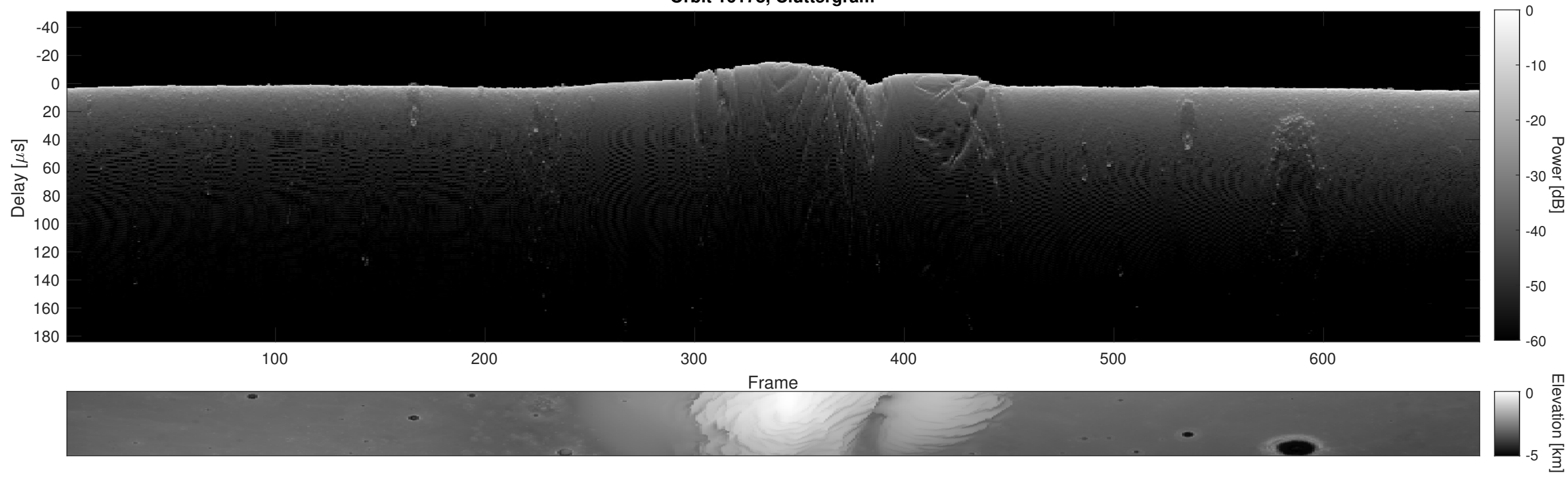
Orbit 16178, Cluttergram
