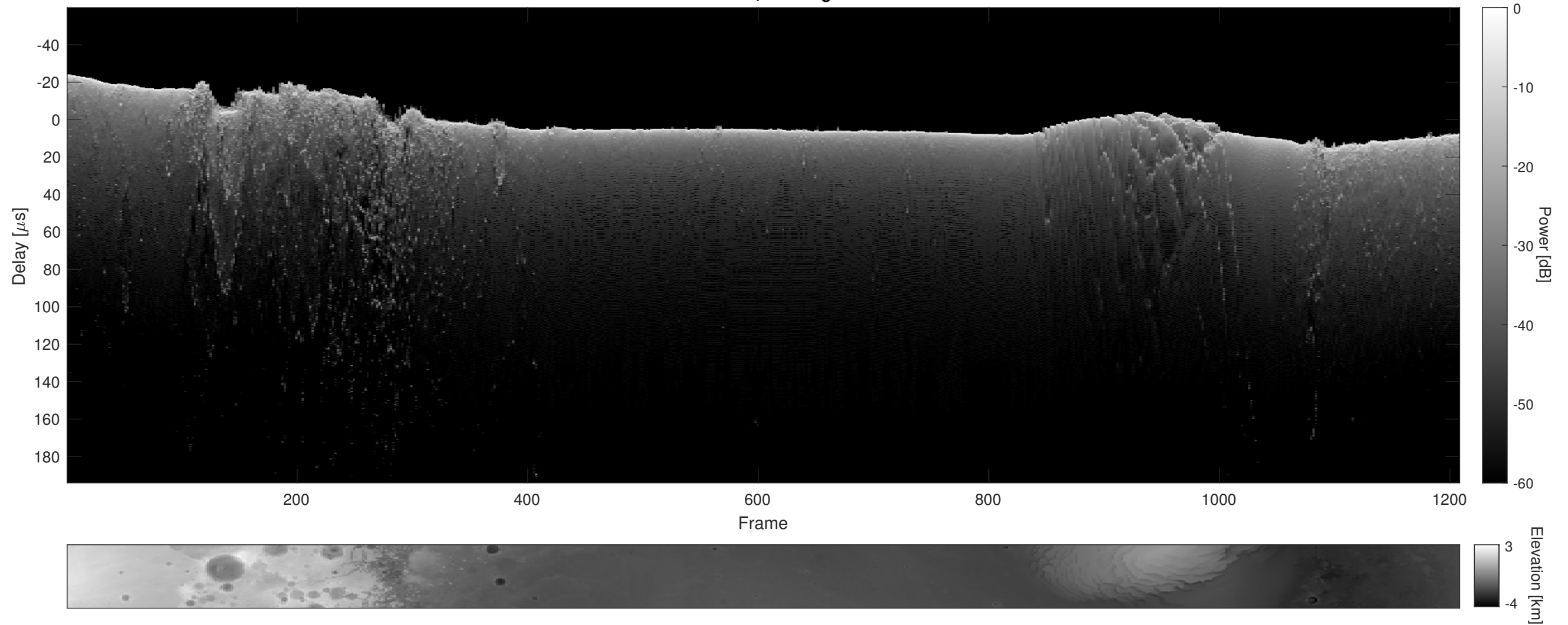
Orbit 16232, Cluttergram
