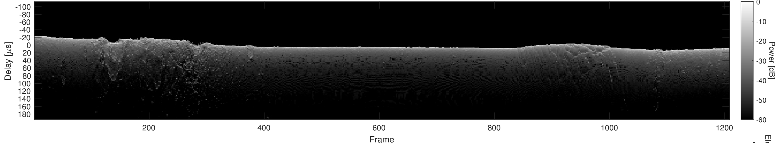
Orbit 16232, Cluttergram
