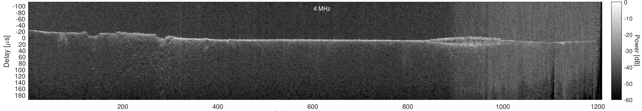
Orbit 16232, Cluttergram
