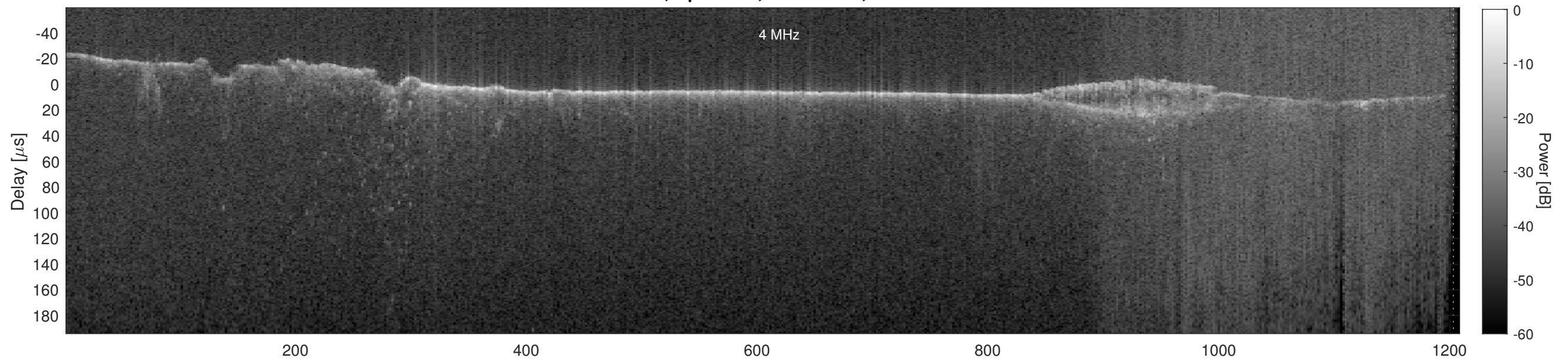
Orbit 16232, Cluttergram
