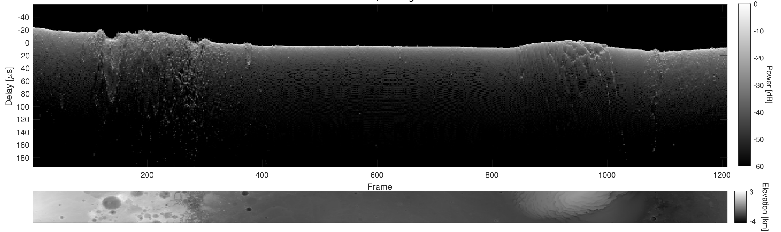
Orbit 16232, Cluttergram
