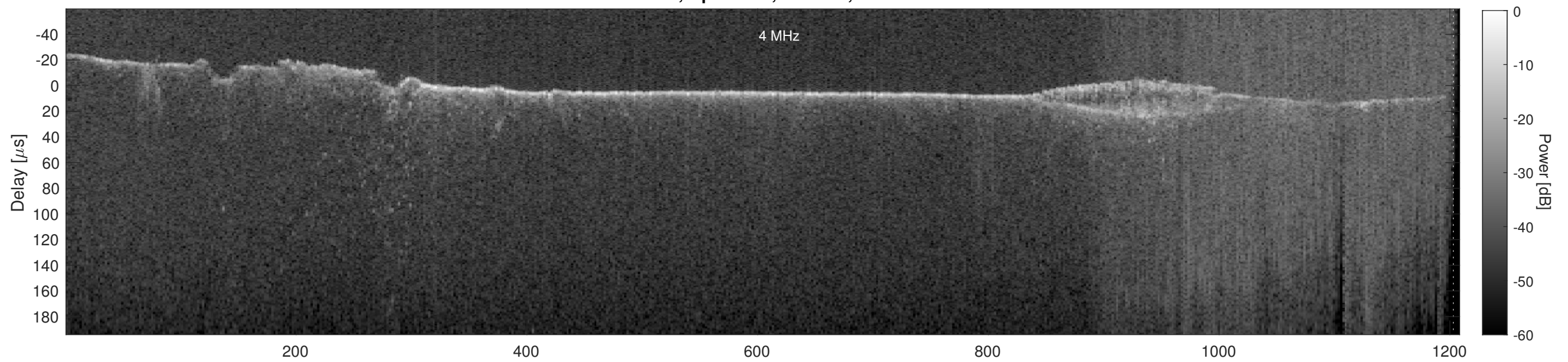
Orbit 16232, Cluttergram
