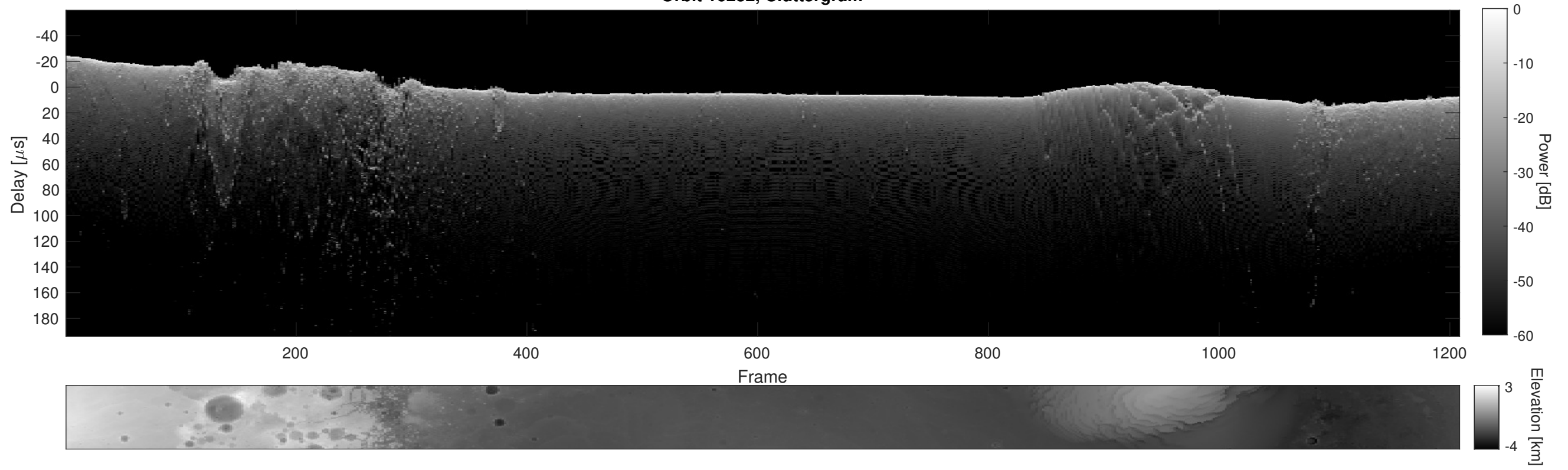
Orbit 16232, Cluttergram
