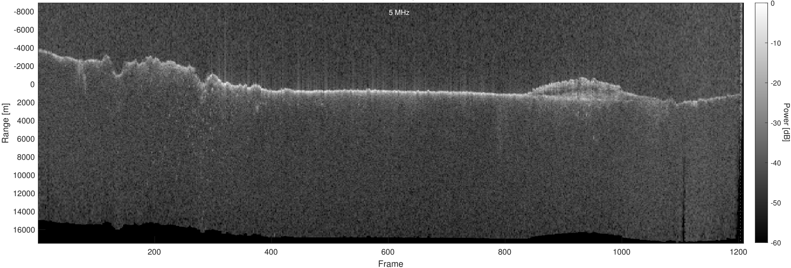
Orbit 16232, Optimized, Window, Depth-Corrected, Channel 2
