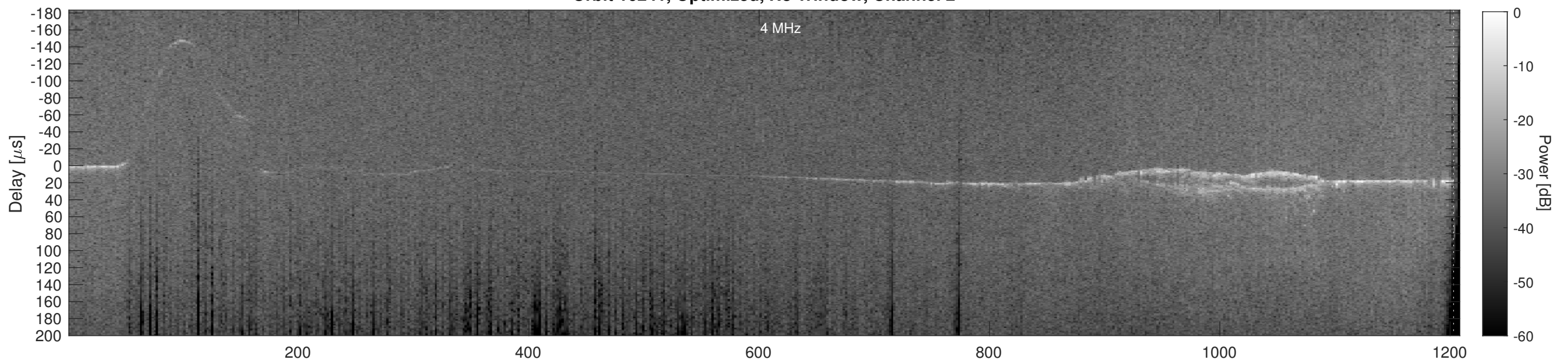
Orbit 16241, Cluttergram
