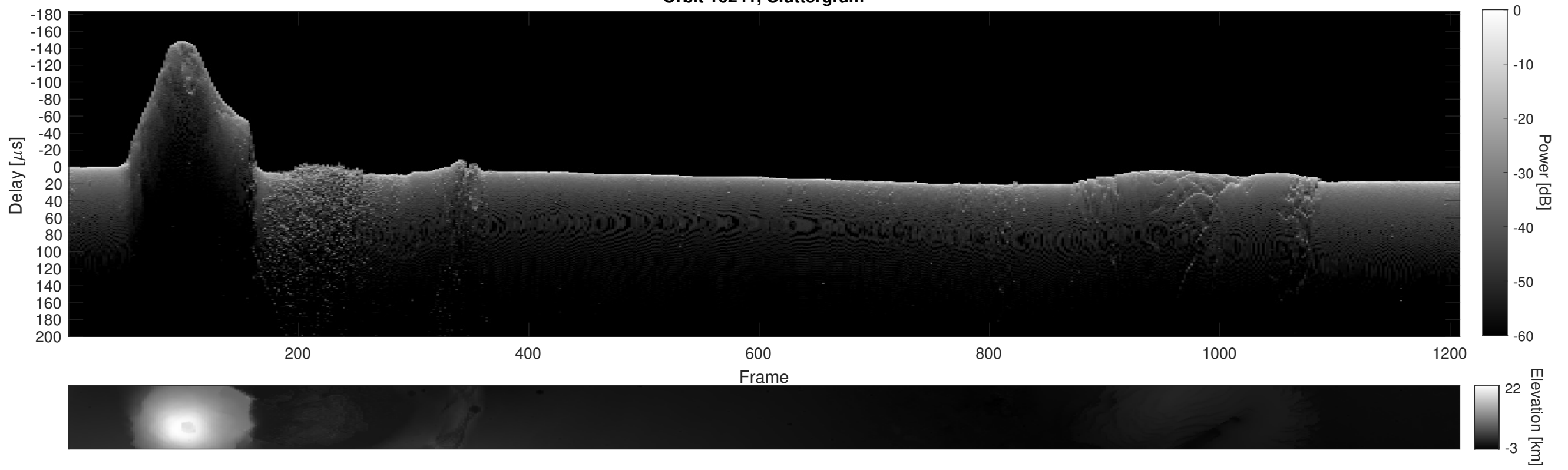
Orbit 16241, Cluttergram
