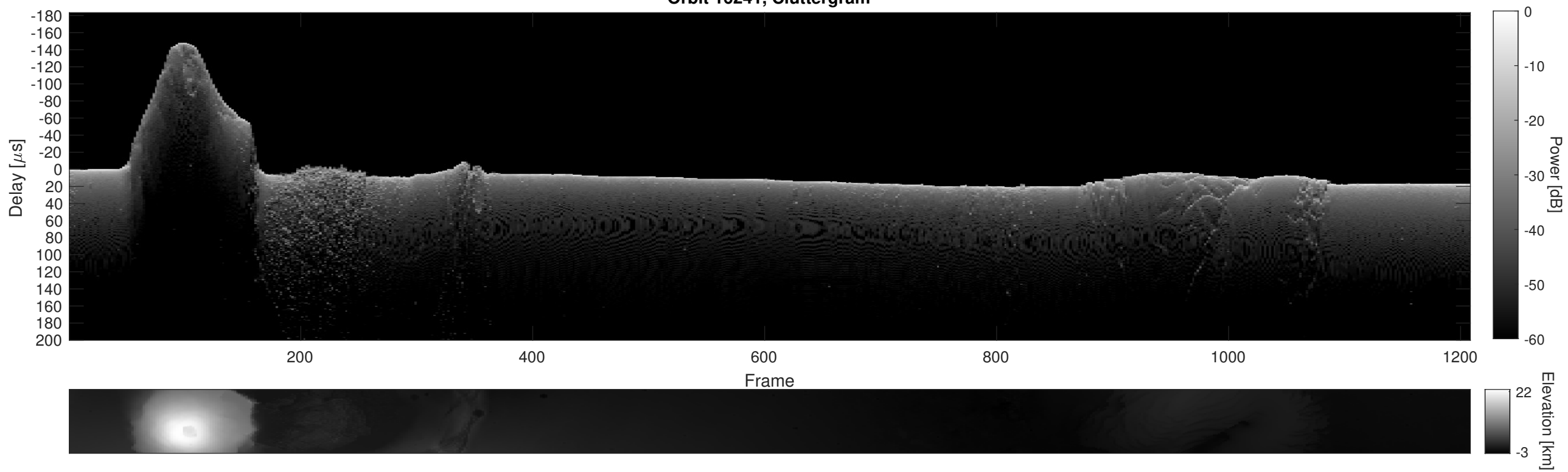
Orbit 16241, Cluttergram
