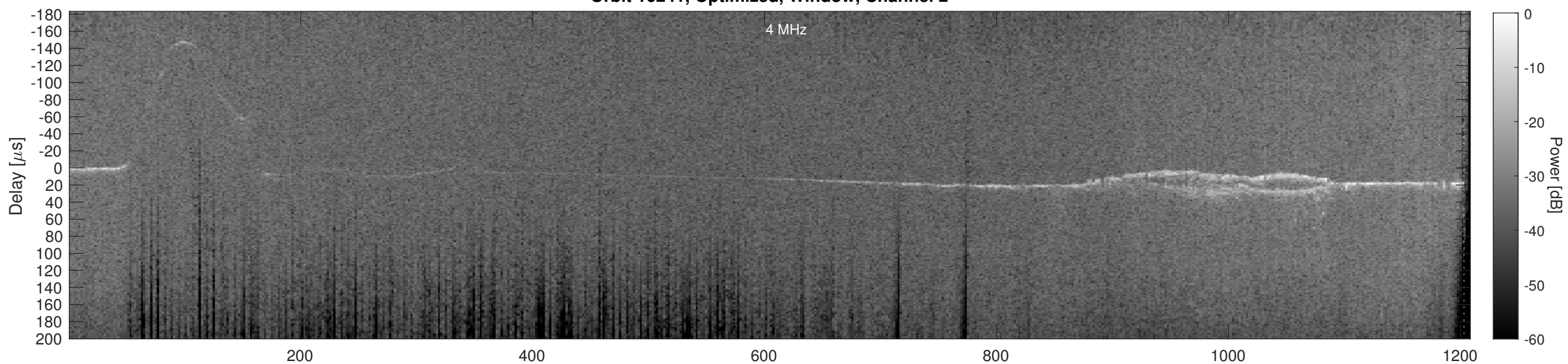
Orbit 16241, Cluttergram
