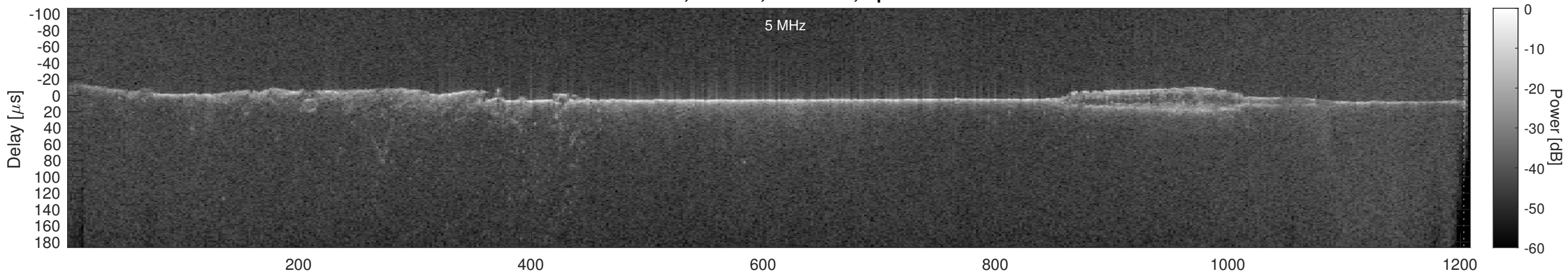
Orbit 16243, Cluttergram
