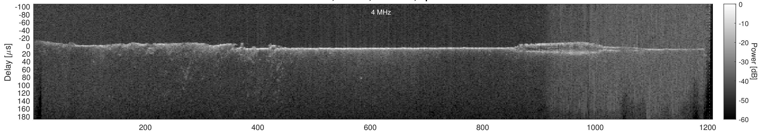
Orbit 16243, Cluttergram
