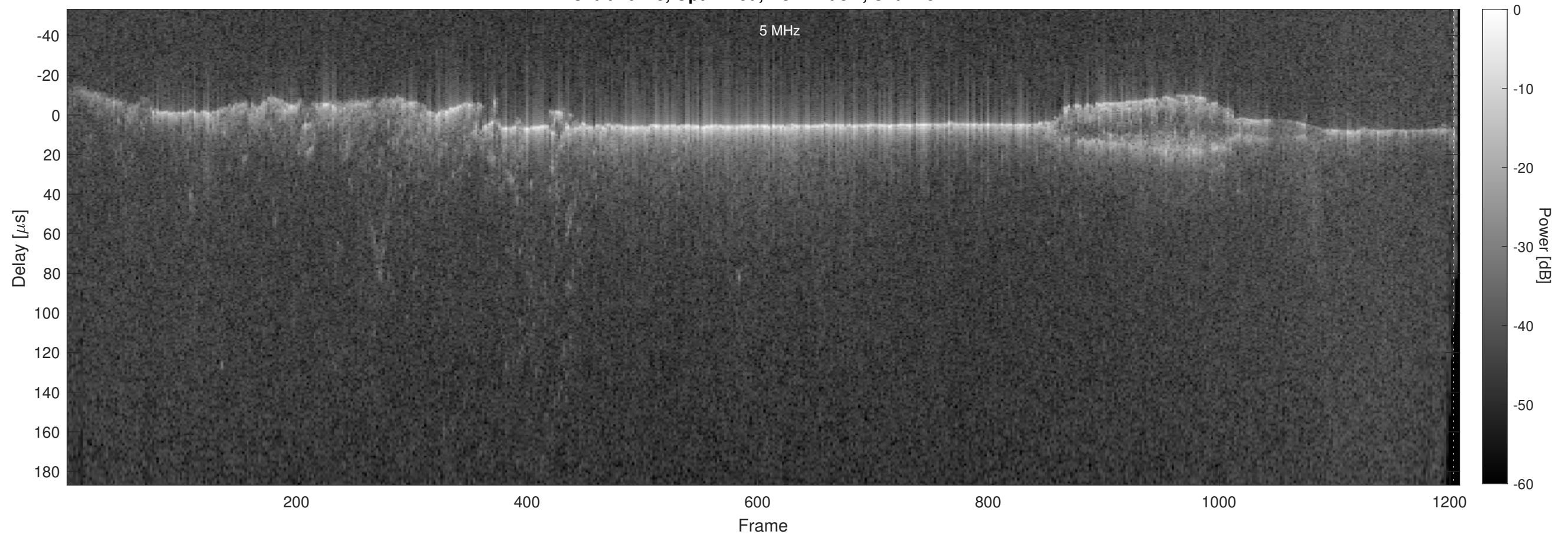
Orbit 16243, Optimized, No Window, Channel 2
