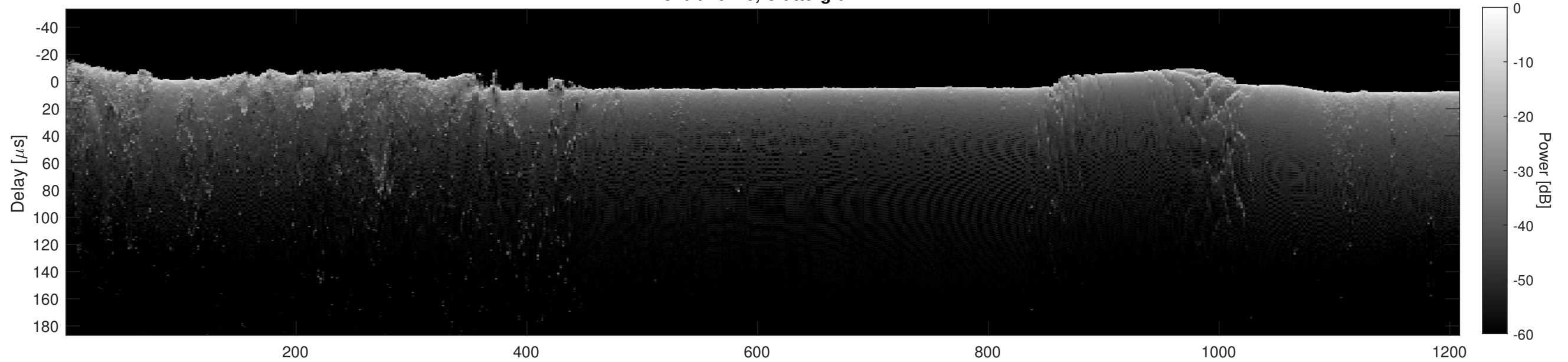
Orbit 16243, Cluttergram
