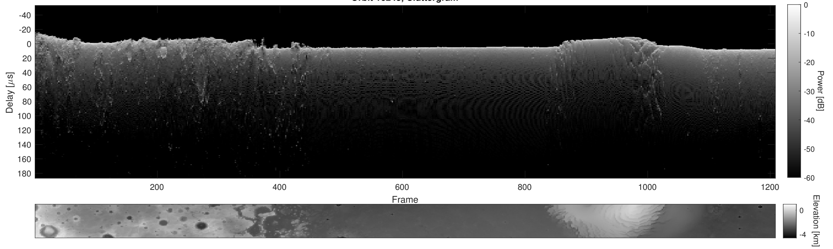
Orbit 16243, Cluttergram
