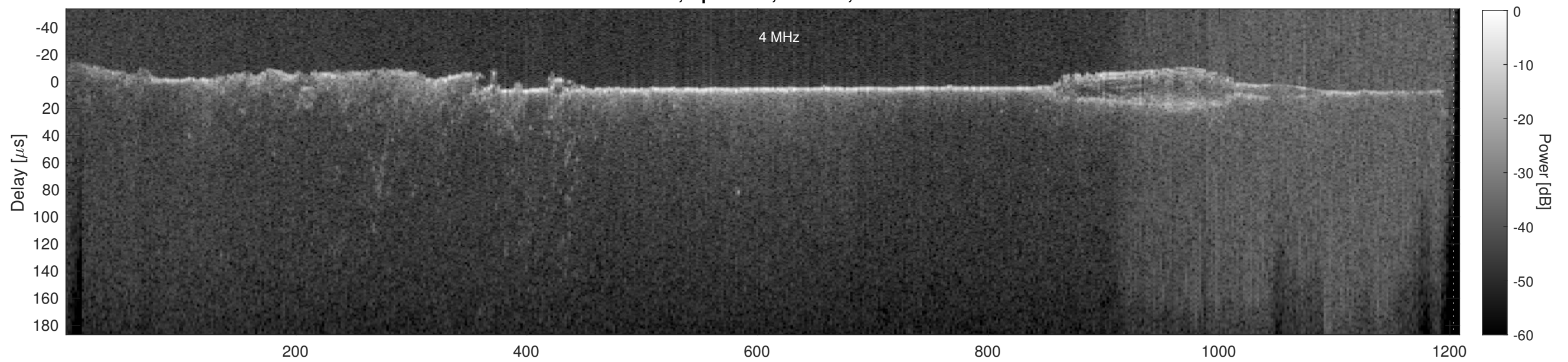
Orbit 16243, Cluttergram
