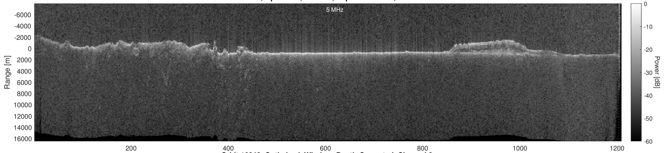
Orbit 16243, Optimized, Window, Depth-Corrected, Channel 2
