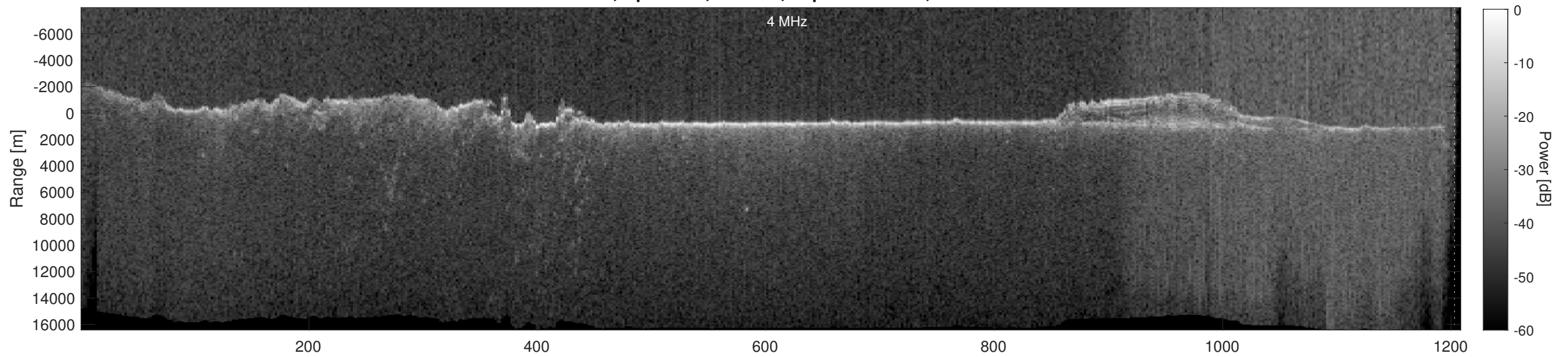
Orbit 16243, Depth-Corrected Cluttergram
