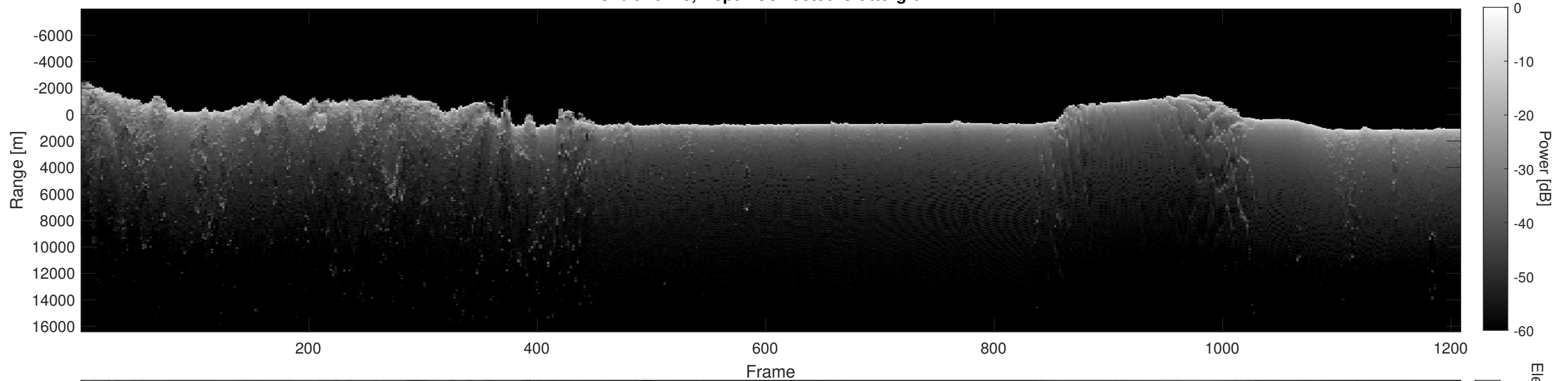
Orbit 16243, Depth-Corrected Cluttergram
