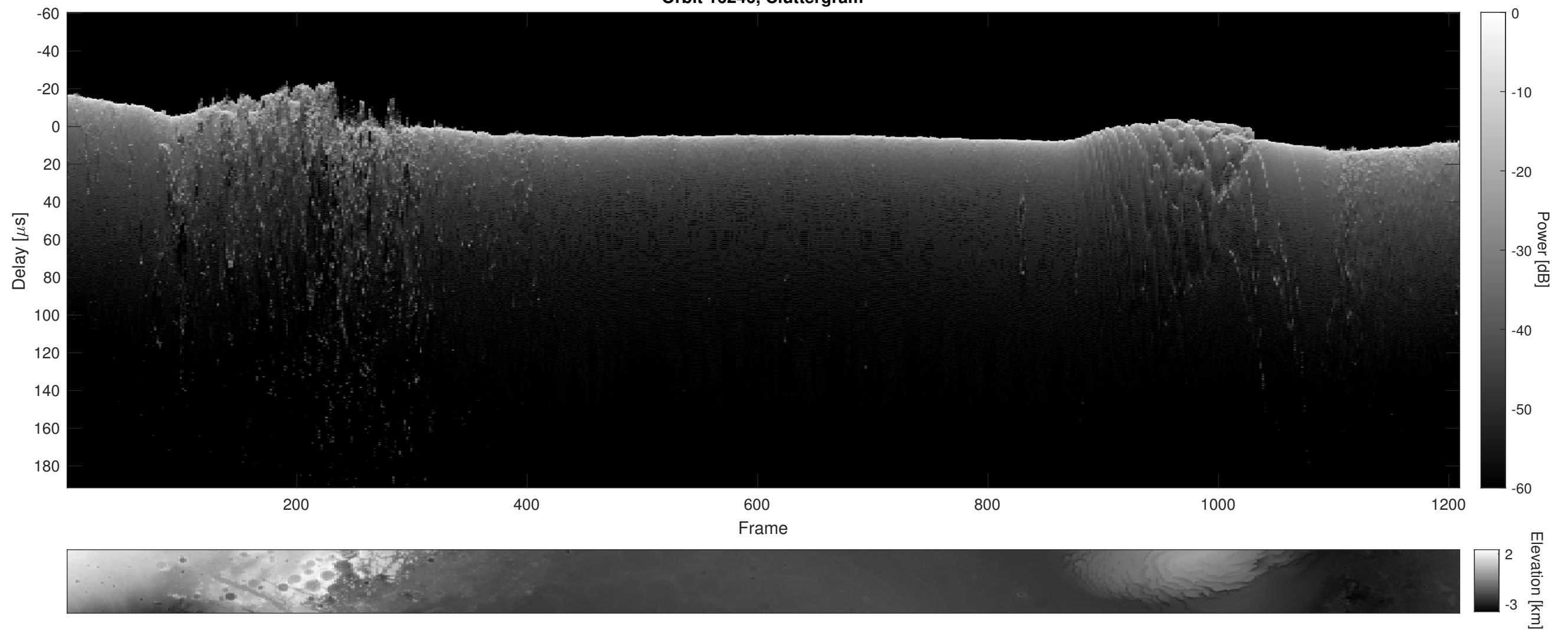
Orbit 16246, Cluttergram
