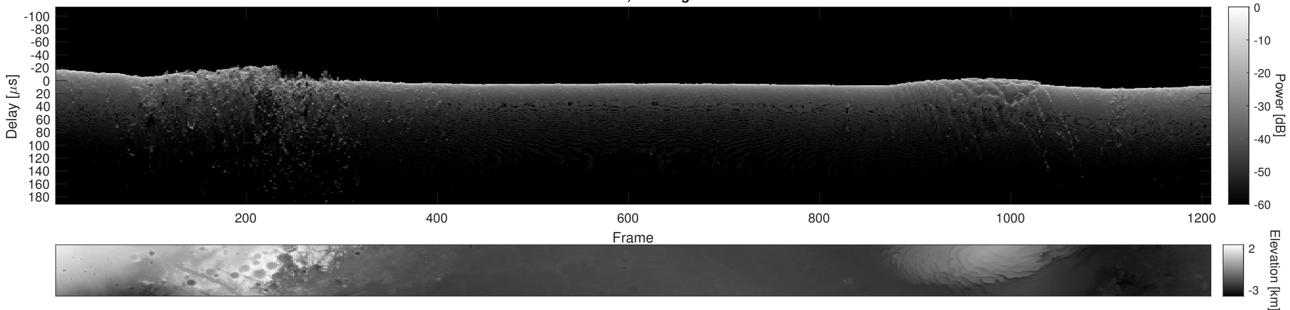
Orbit 16246, Cluttergram
