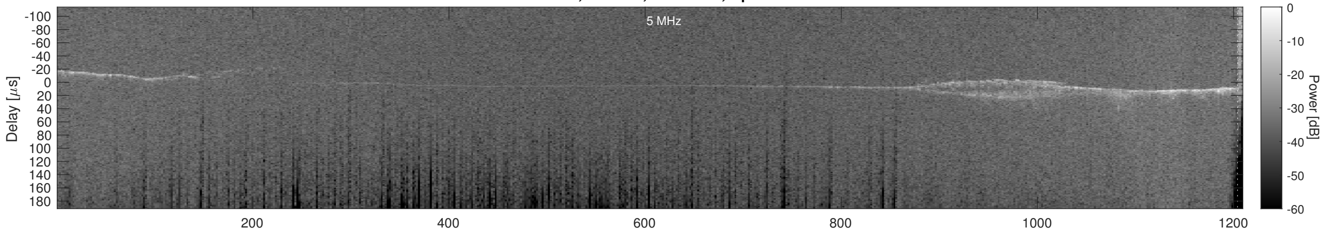
Orbit 16246, Cluttergram
