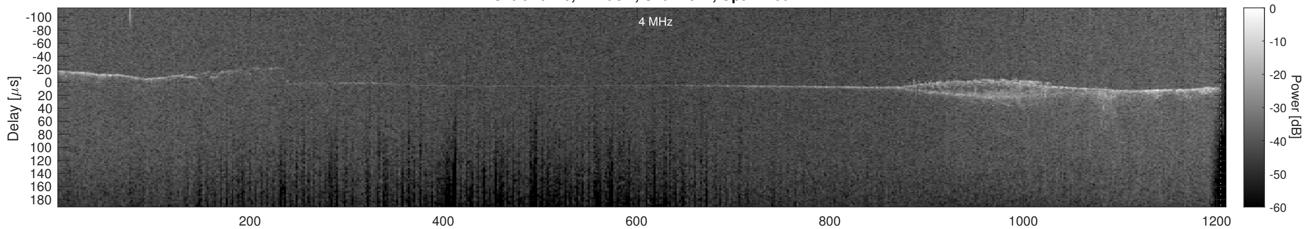
Orbit 16246, Cluttergram
