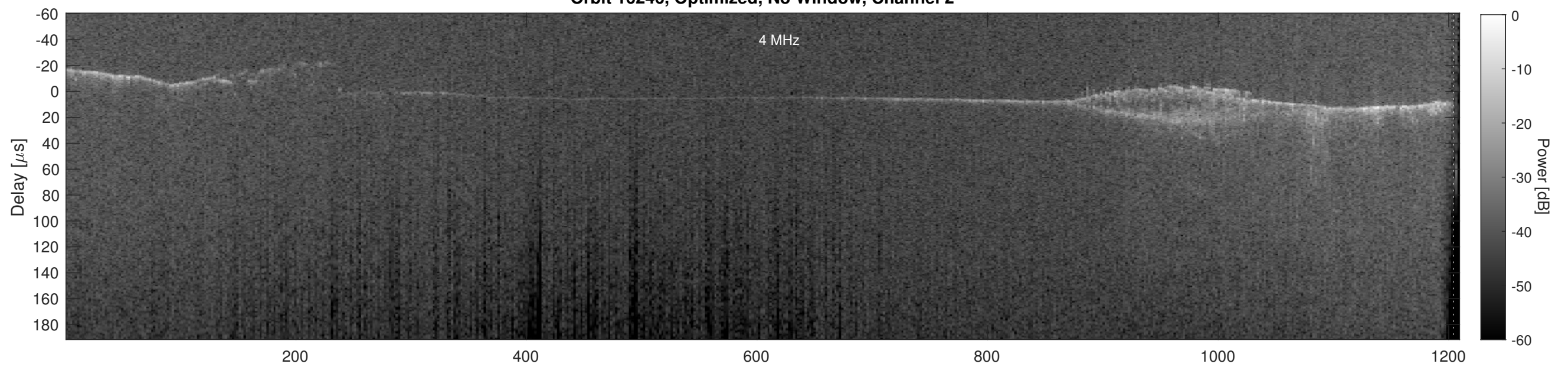
Orbit 16246, Cluttergram
