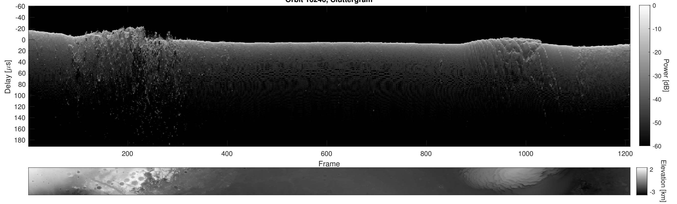
Orbit 16246, Cluttergram
