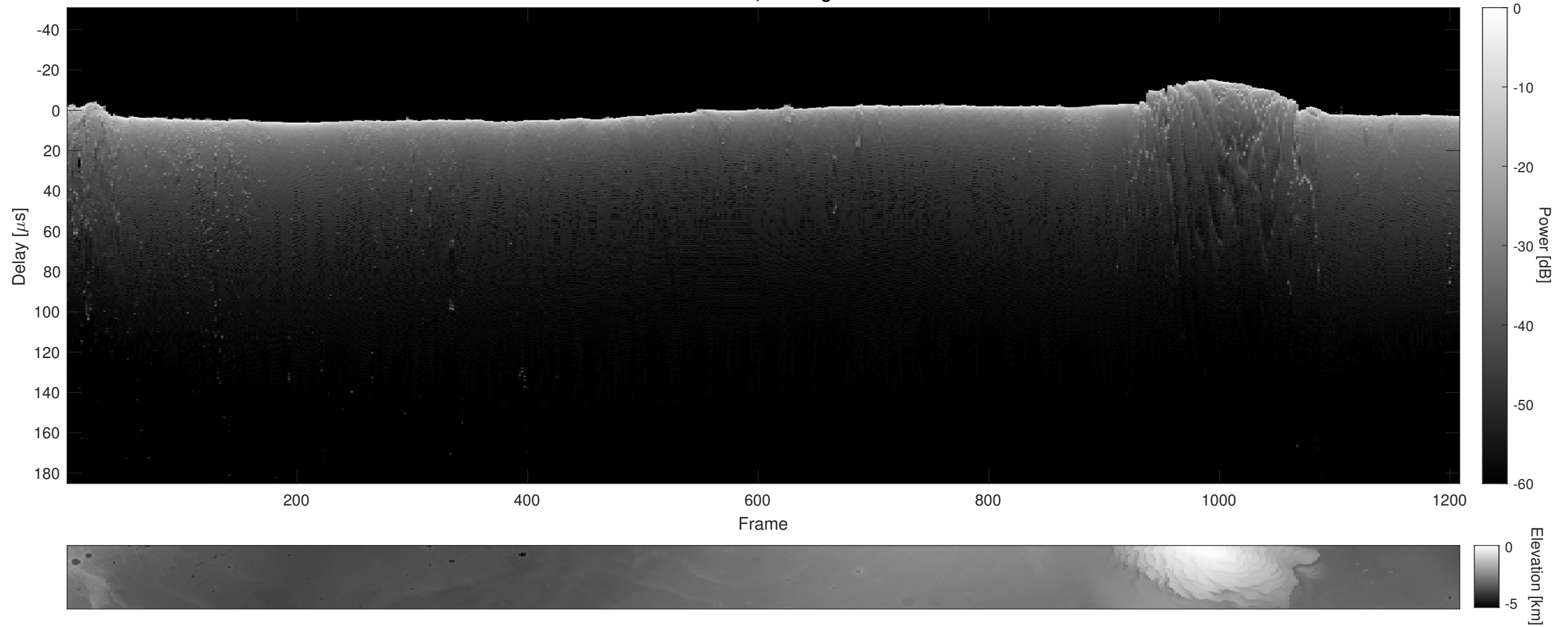
Orbit 16249, Cluttergram
