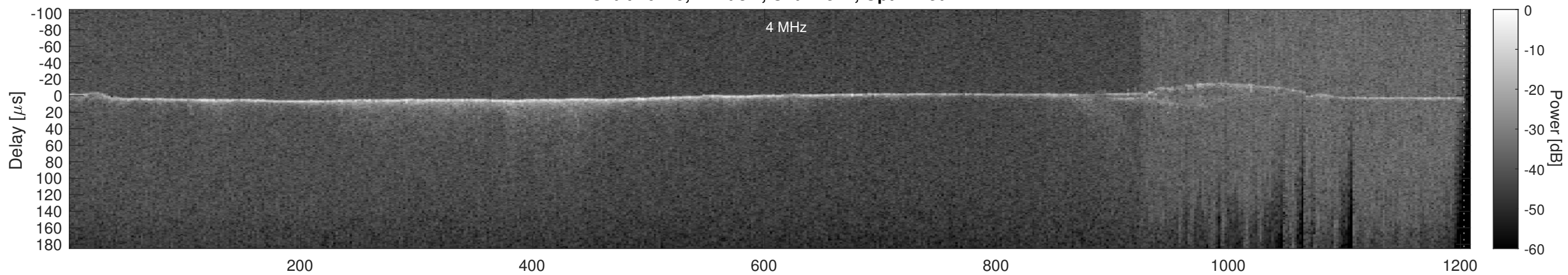
Orbit 16249, Cluttergram
