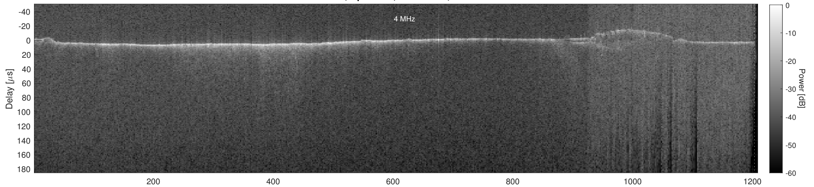
Orbit 16249, Cluttergram
