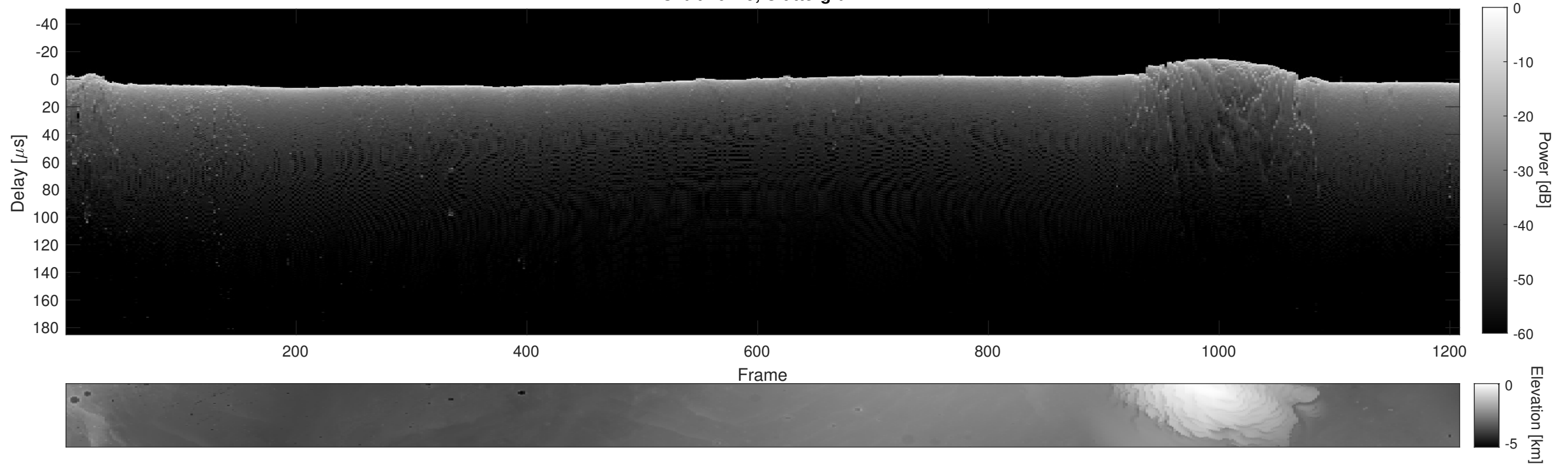
Orbit 16249, Cluttergram
