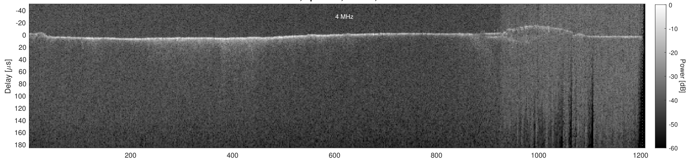
Orbit 16249, Cluttergram
