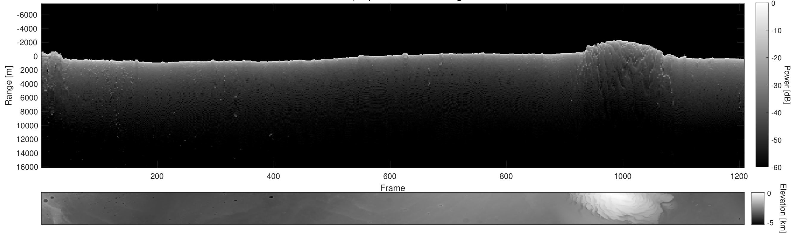
Orbit 16249, Depth-Corrected Cluttergram
