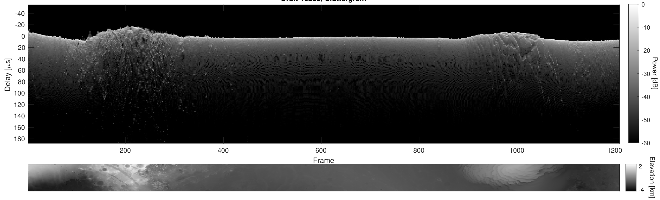
Orbit 16253, Cluttergram
