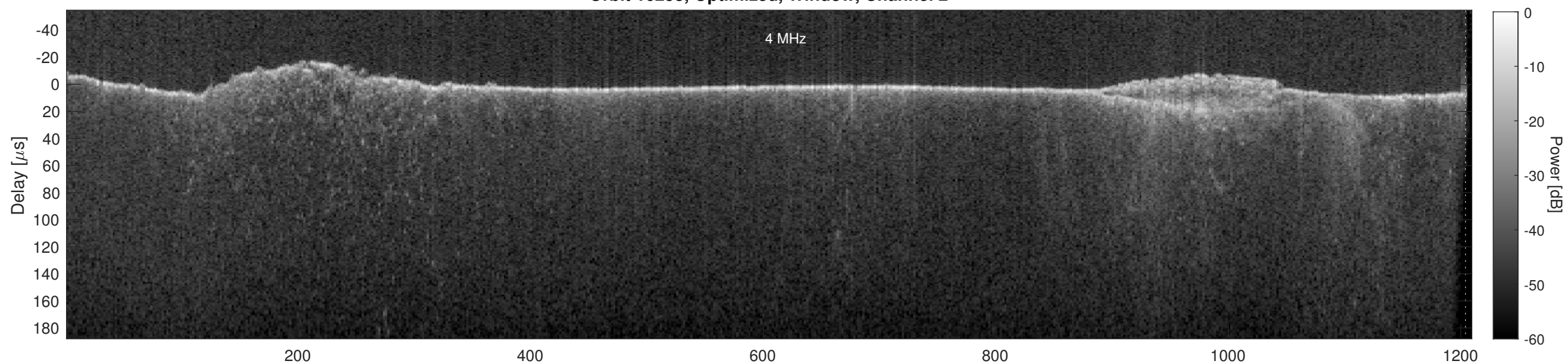
Orbit 16253, Cluttergram
