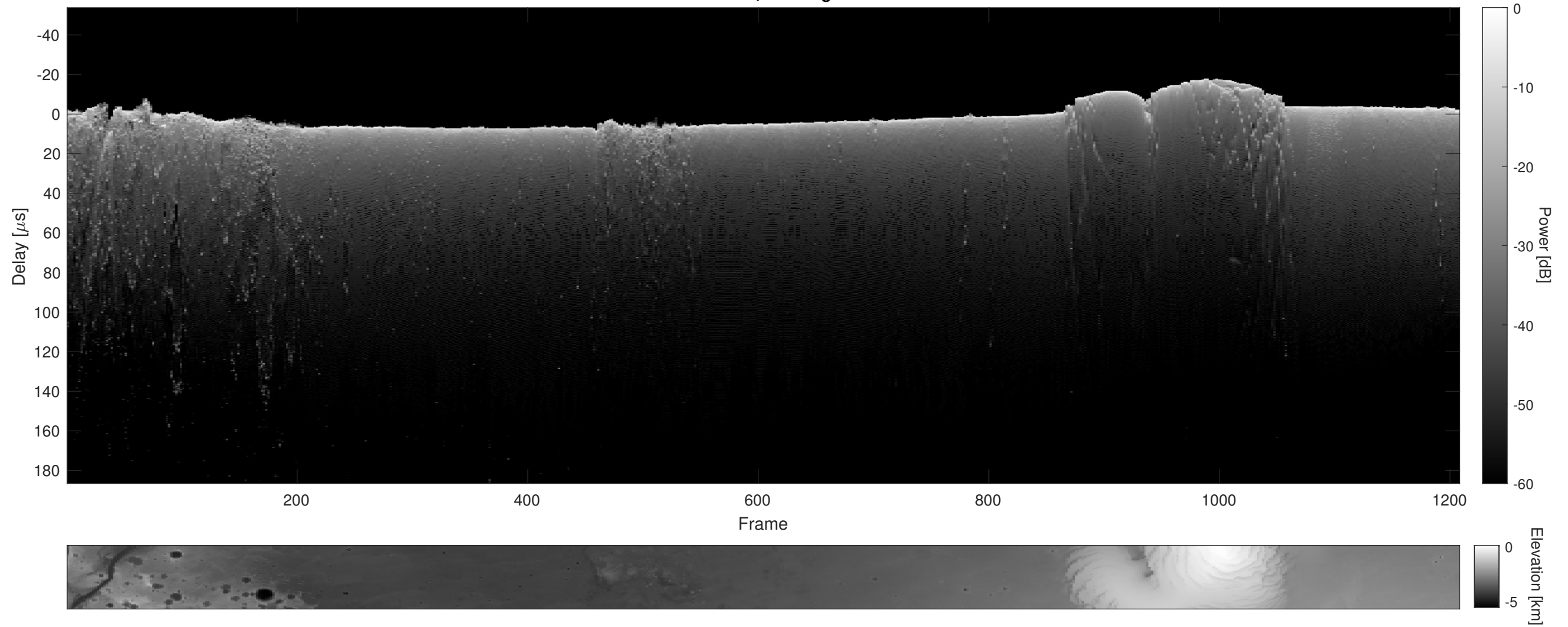
Orbit 16254, Cluttergram
