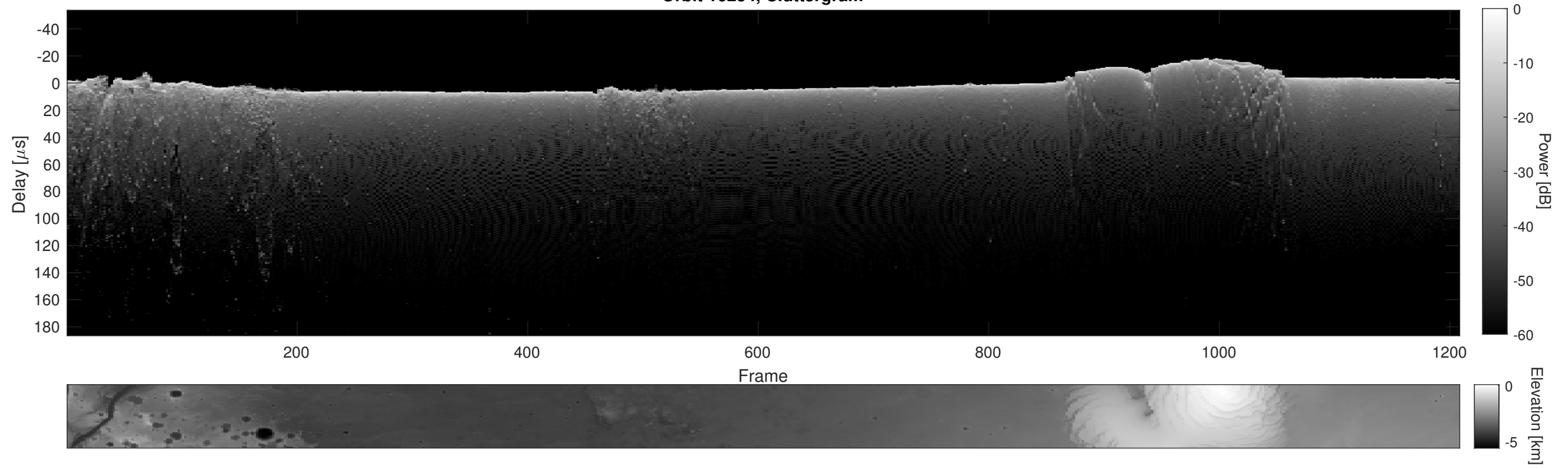
Orbit 16254, Cluttergram
