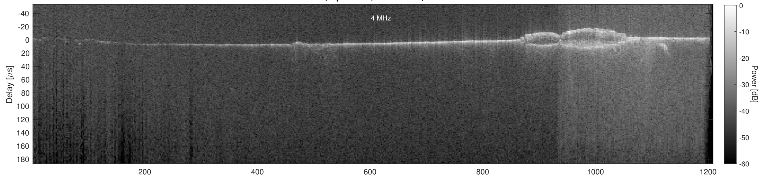
Orbit 16254, Cluttergram
