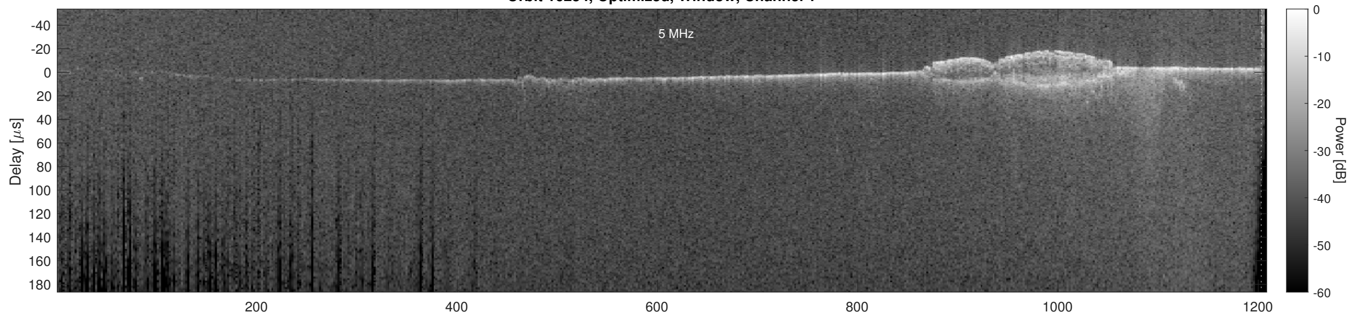
Orbit 16254, Optimized, Window, Channel 2
