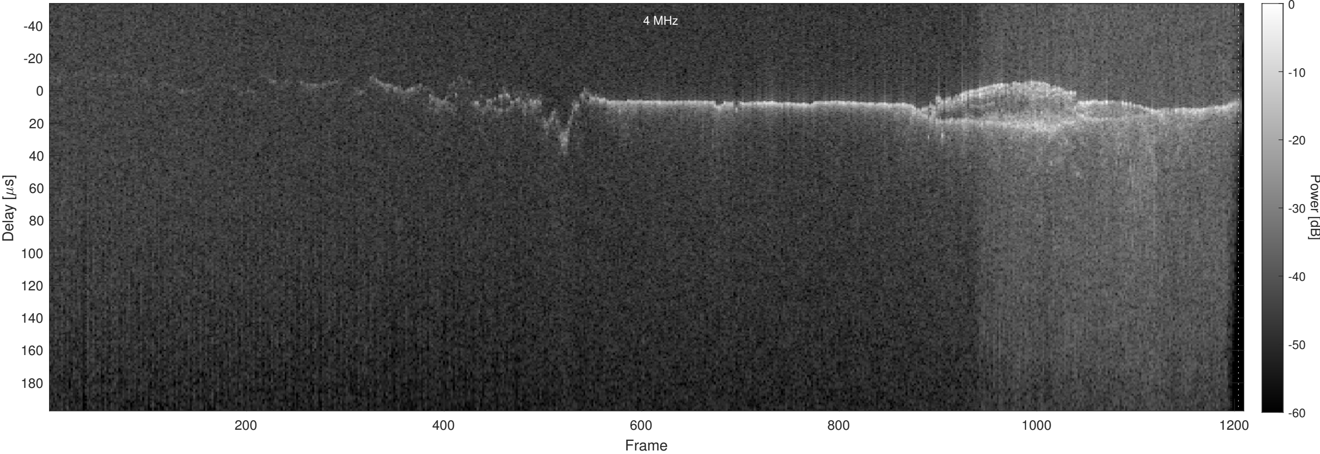
Orbit 16257, Chapman, No Window, Channel 2
