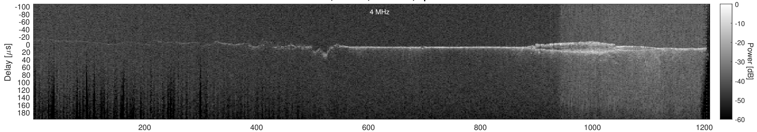
Orbit 16257, Cluttergram
