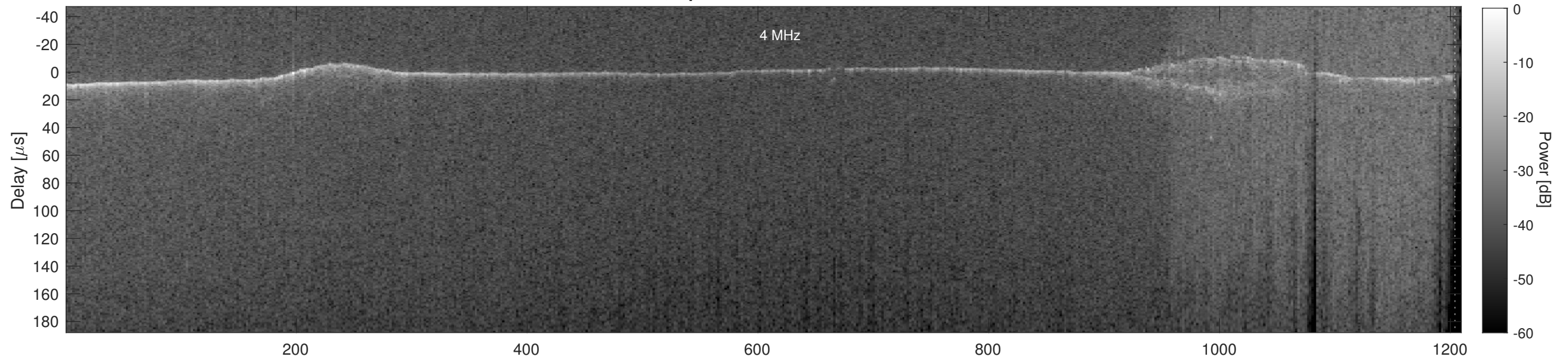
Orbit 16267, Cluttergram
