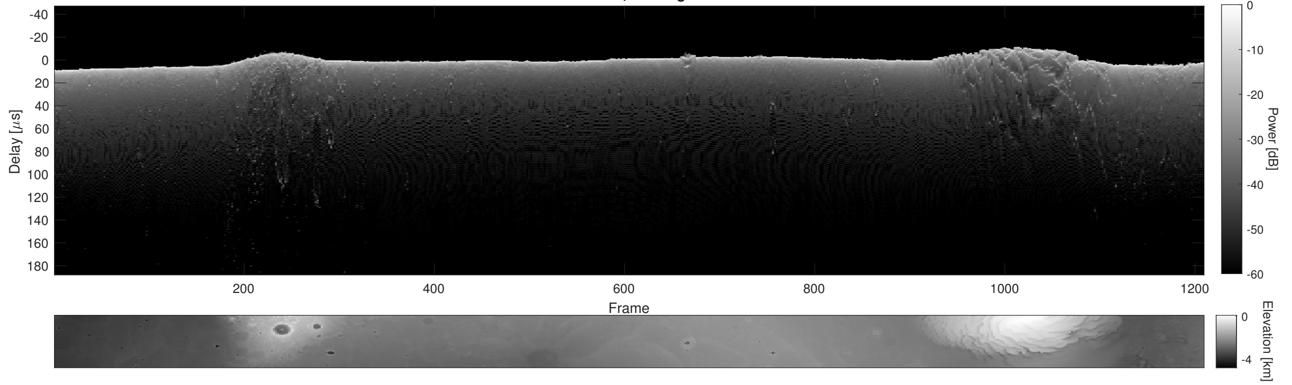
Orbit 16267, Cluttergram
