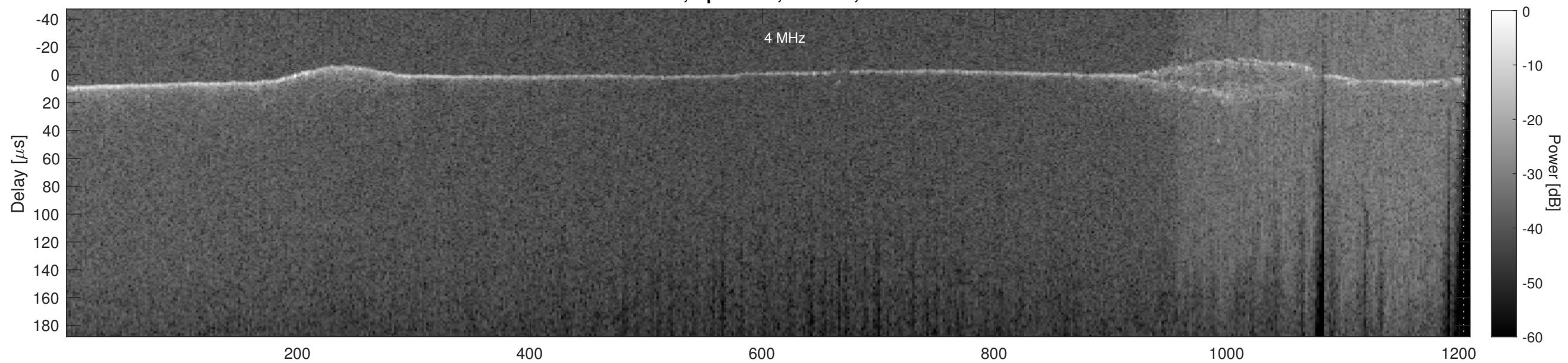
Orbit 16267, Cluttergram
