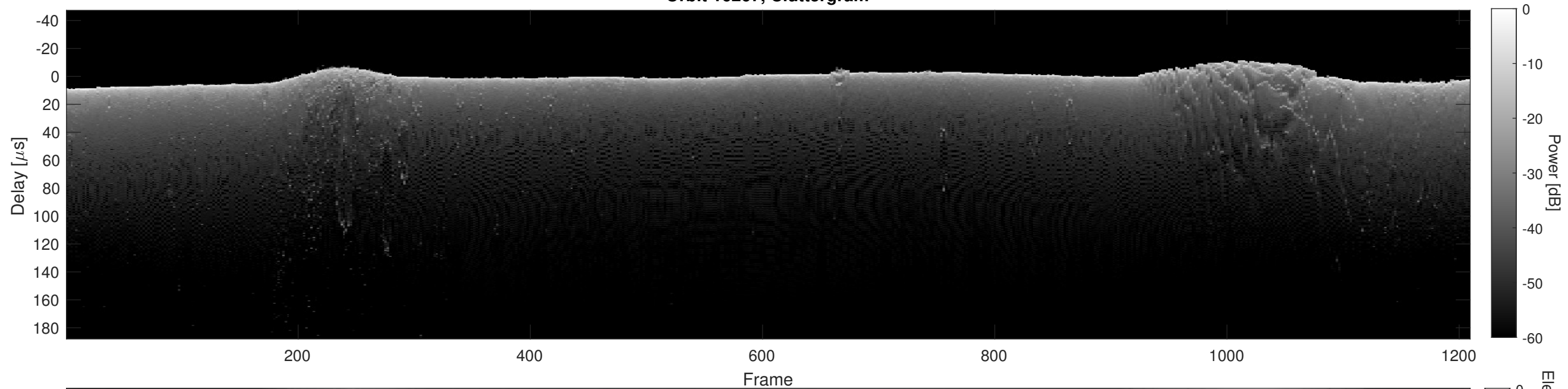
Orbit 16267, Cluttergram
