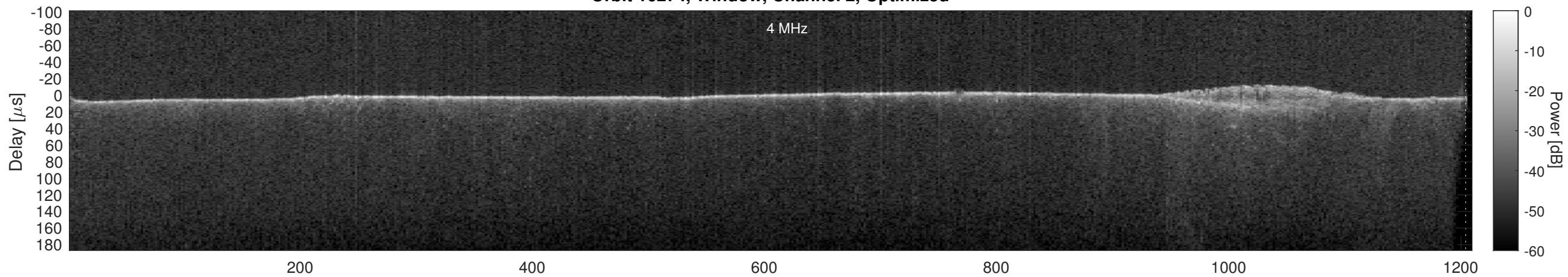
Orbit 16274, Cluttergram
