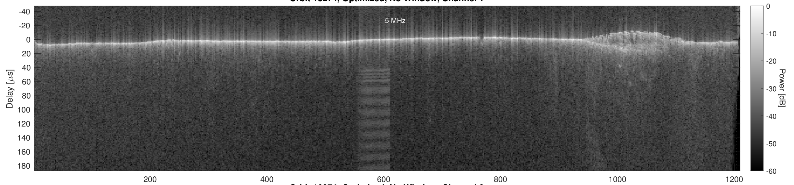
Orbit 16274, Optimized, No Window, Channel 2
