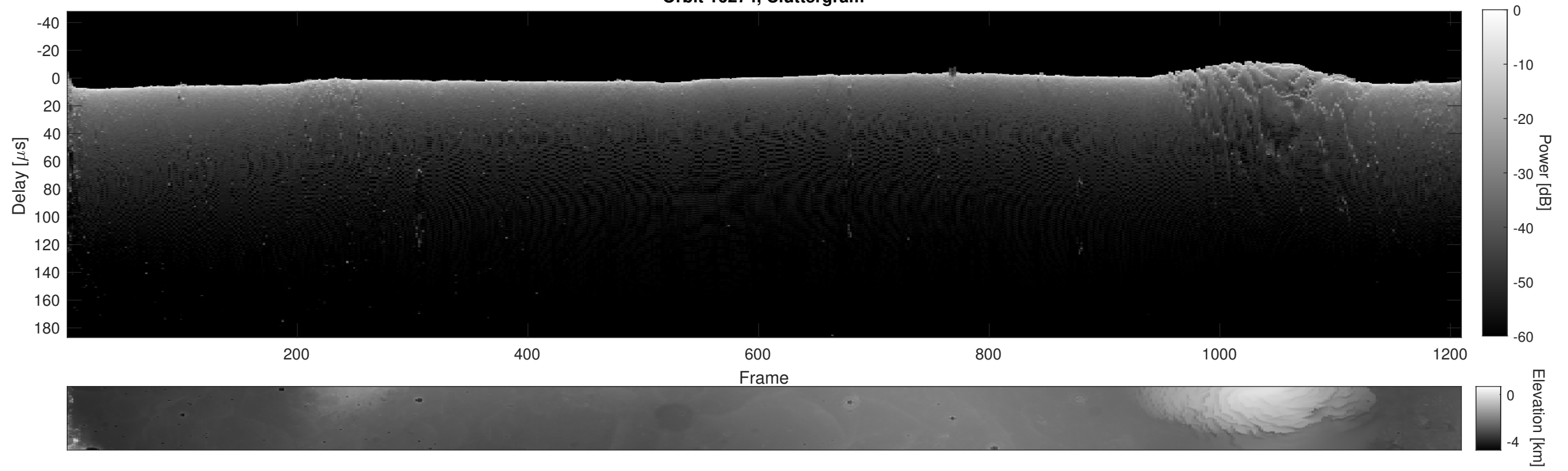
Orbit 16274, Cluttergram
