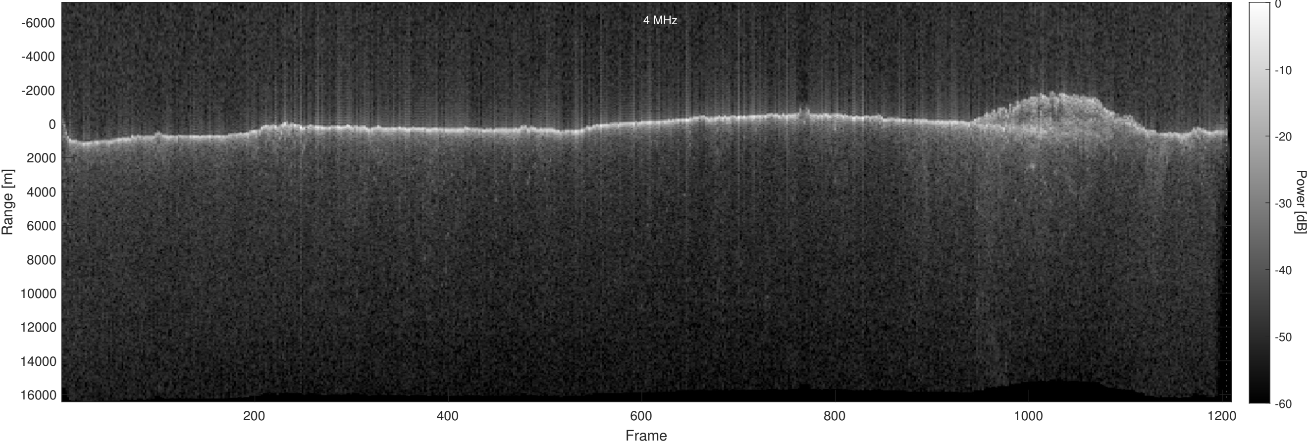
Orbit 16274, Optimized, No Window, Depth-Corrected, Channel 2
