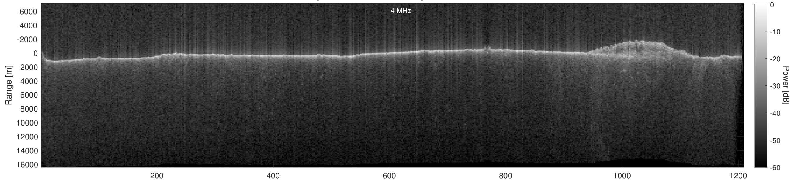
Orbit 16274, Depth-Corrected Cluttergram
