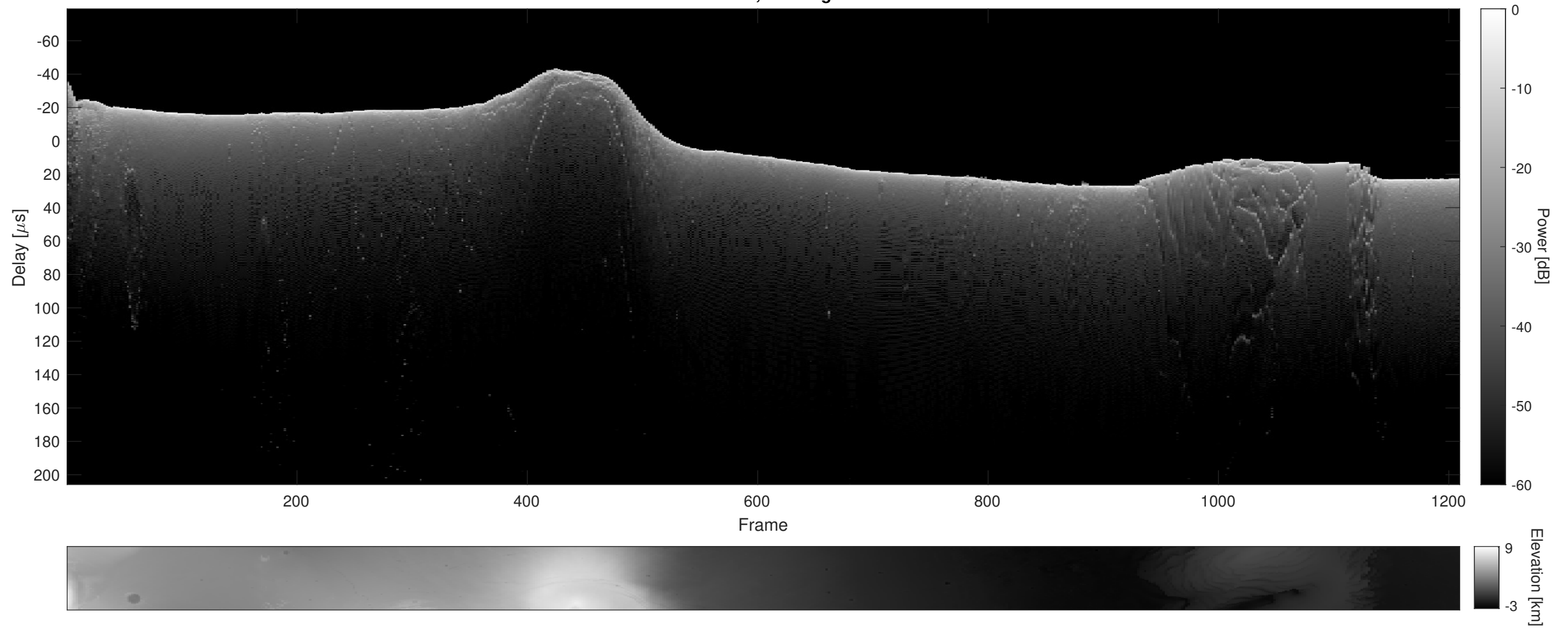
Orbit 16276, Cluttergram
