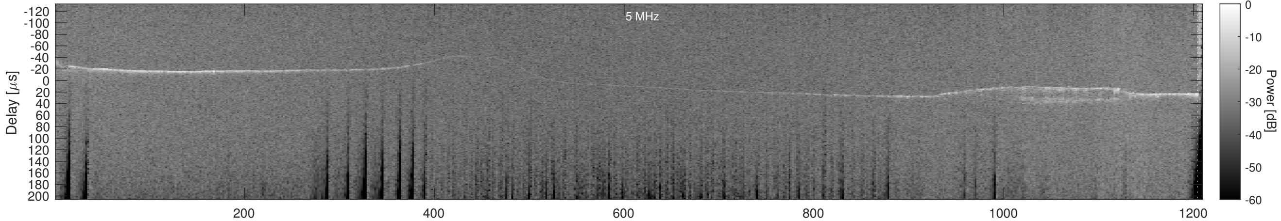
Orbit 16276, Cluttergram
