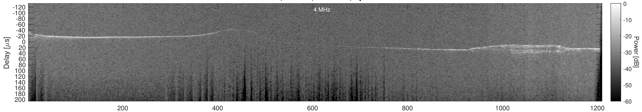
Orbit 16276, Cluttergram
