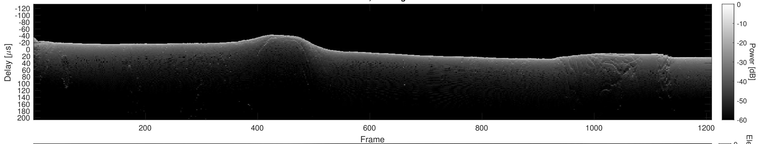
Orbit 16276, Cluttergram
