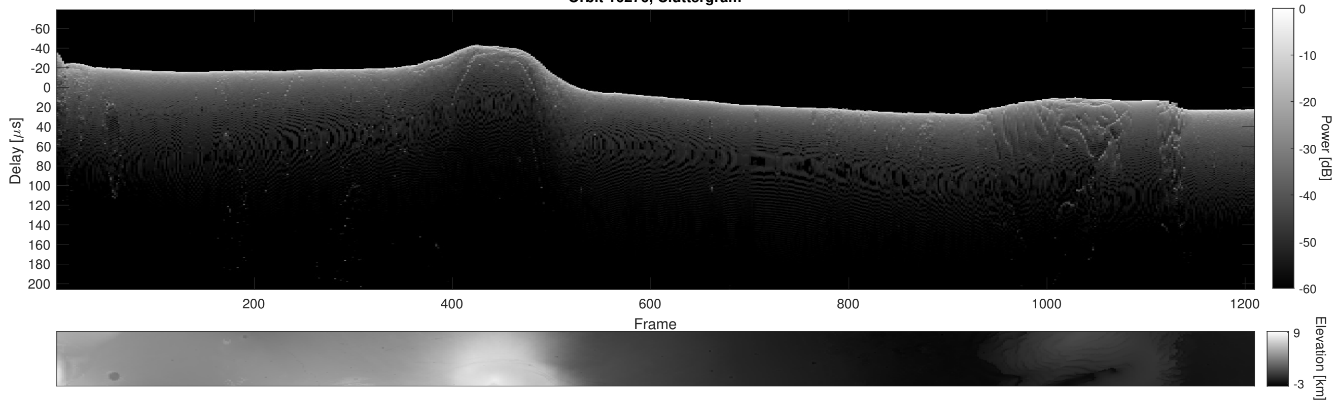
Orbit 16276, Cluttergram
