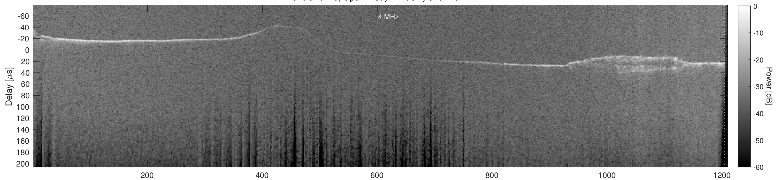
Orbit 16276, Cluttergram
