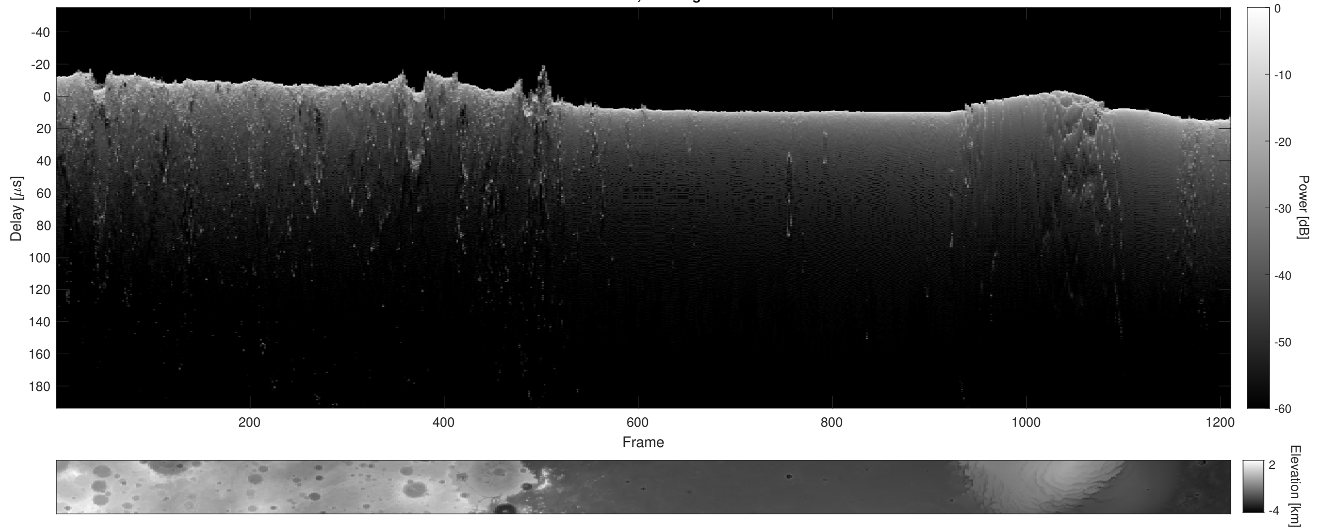
Orbit 16278, Cluttergram
