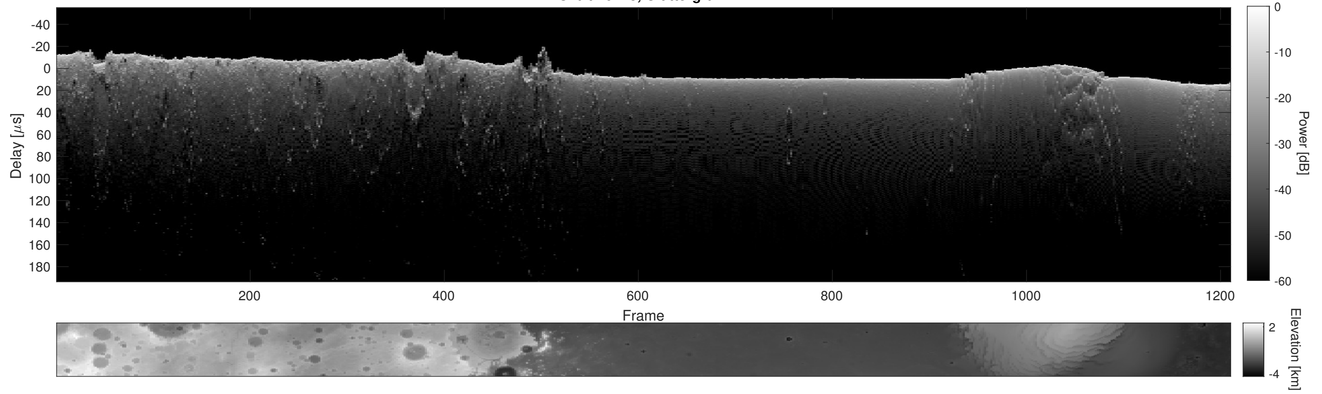
Orbit 16278, Cluttergram
