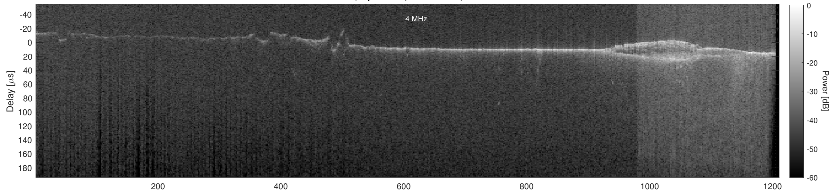
Orbit 16278, Cluttergram
