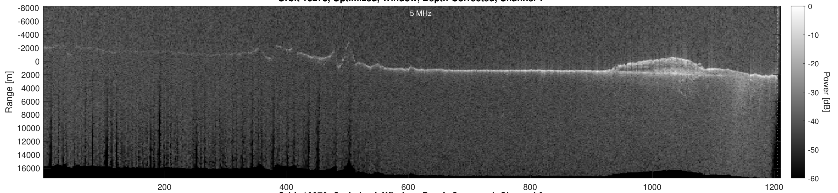
Orbit 16278, Optimized, Window, Depth-Corrected, Channel 2
