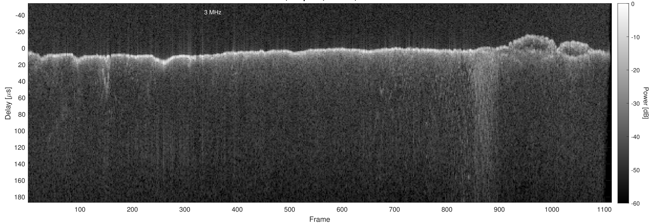
Orbit 16280, Chapman, Window, Channel 2
