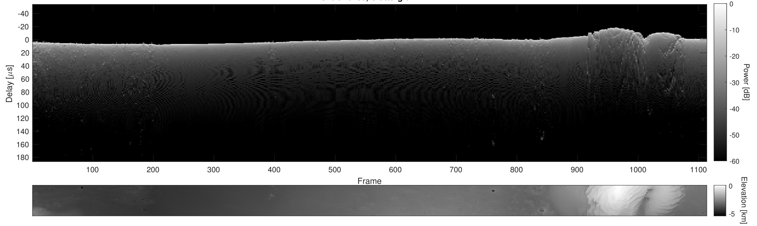
Orbit 16280, Cluttergram
