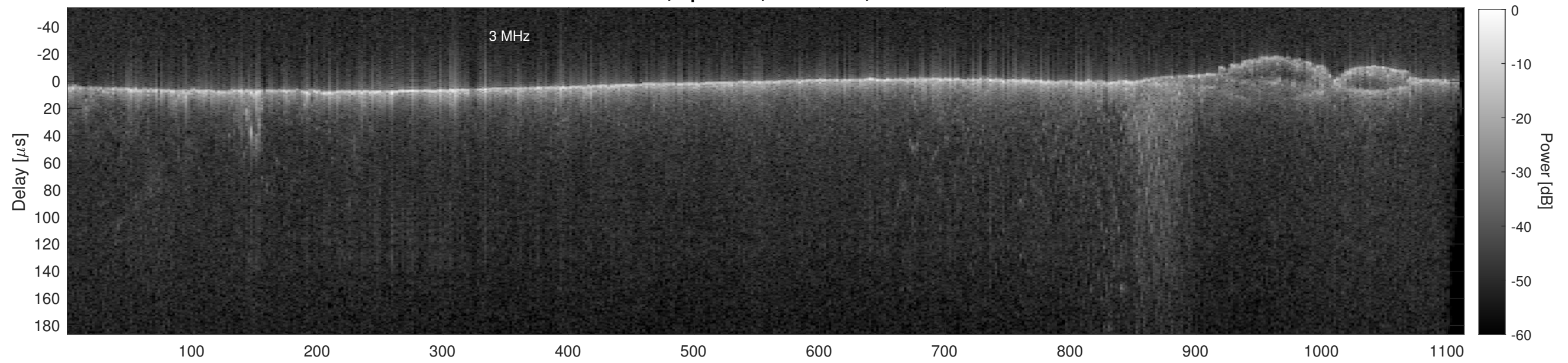
Orbit 16280, Cluttergram
