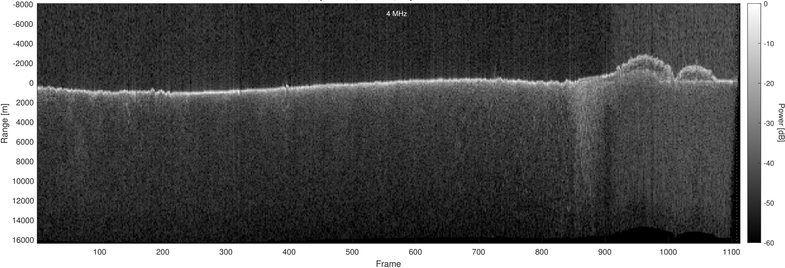
Orbit 16280, Optimized, Window, Depth-Corrected, Channel 2
