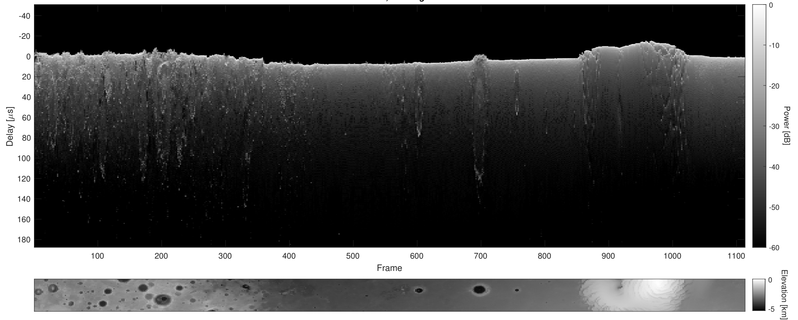
Orbit 16282, Cluttergram
