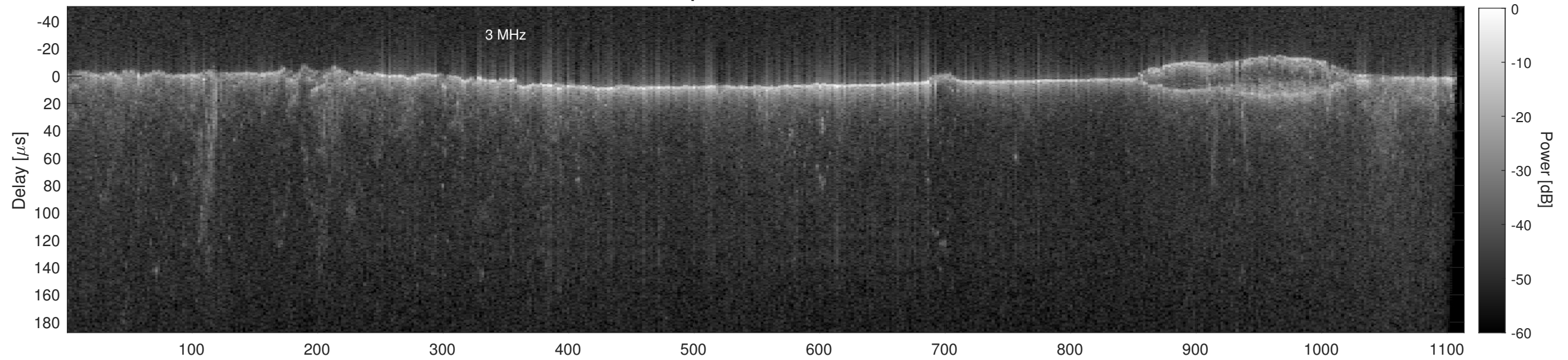
Orbit 16282, Cluttergram
